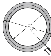
Sealing ring VMAT186375A P for Ø75 tubes
