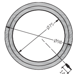
Sealing ring VMAT187590A P for Ø90 tubes
